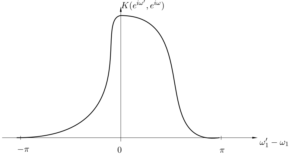
Fig. 1: Weighting kernel Spillovers across geography can be asymmetric and unimodal. Section through K shown has \omega' = (\omega'_1, \omega'_2) and \omega = (\omega_1, \omega_2) , with \omega'_2 and \omega_2 fixed.
