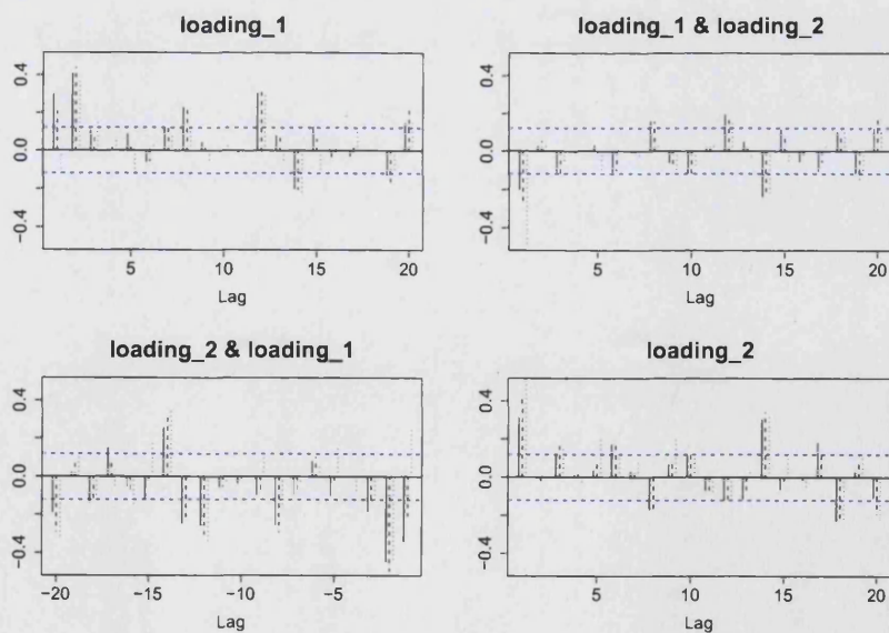
Figure 1.9: PACF of \hat{\eta}_{tj} using bandwidths h = 0.5\hat{h}_t (solid lines), \hat{h}_t (dashed lines) and 2\hat{h}_t (dotted lines).
