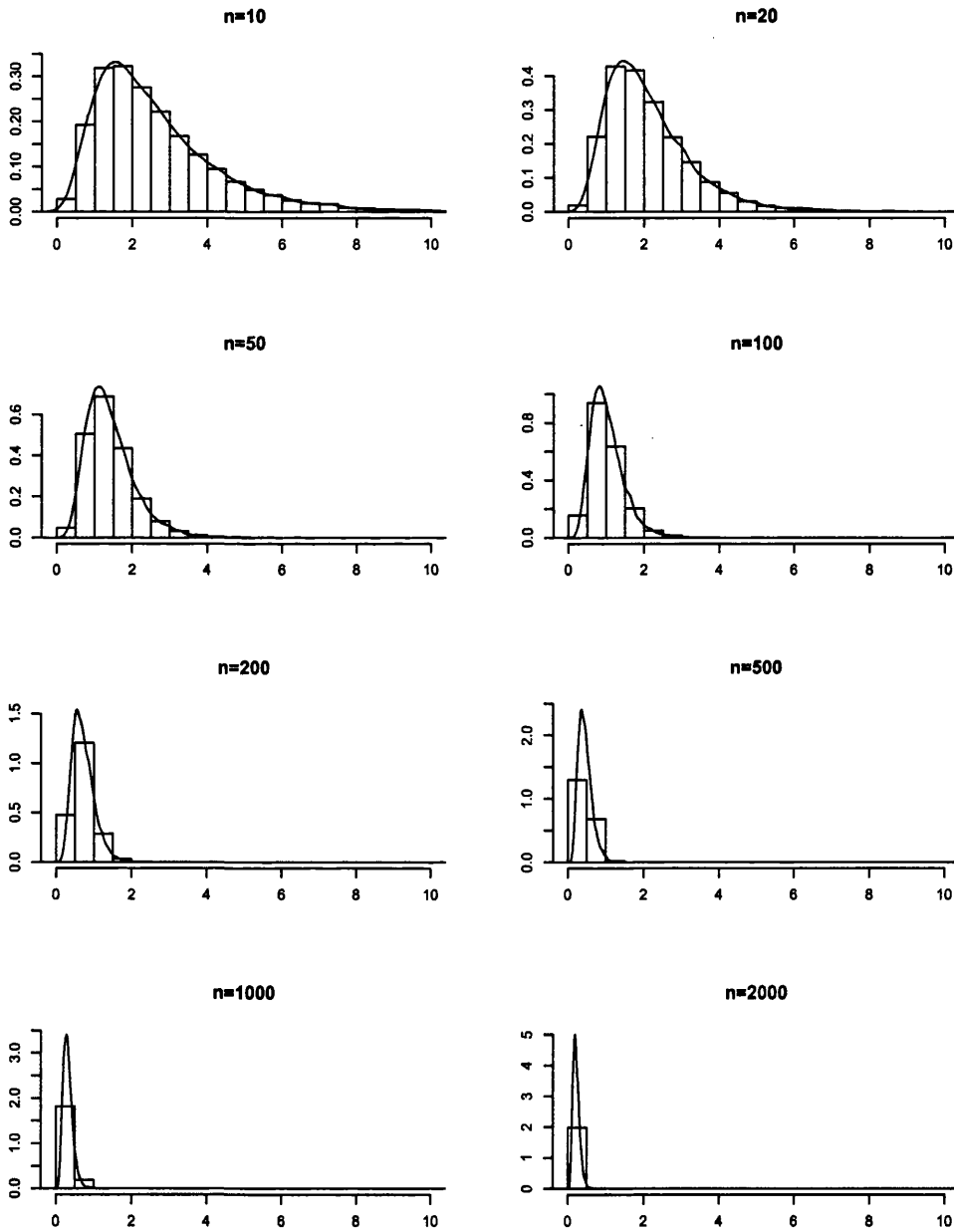
Figure 2.3: Histograms overlaid by kernel density estimates of \sqrt{n}\hat{\lambda}_2 .
