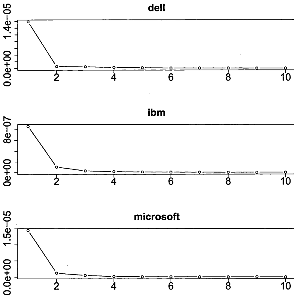
Figure 2.9: Ten largest eigenvalues of \widehat{L}_q .
