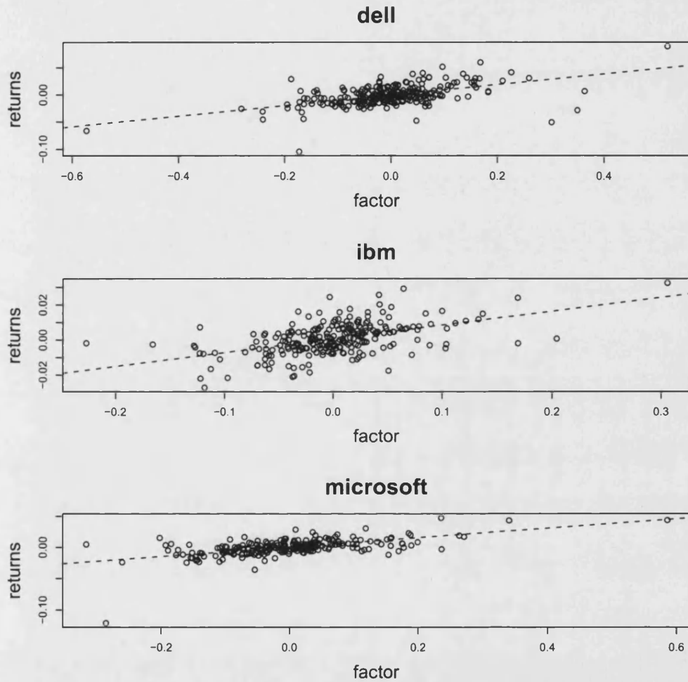
Figure 2.11: Scatter plots of the stocks returns R_t against the estimated common factor Z_{t1} = \mathbf{Y}'_t \hat{\mathbf{e}}_1 . The period is 04/01/2006 - 29/12/2006. The dashed line represents an estimate of the regression R_t = \alpha + \beta Z_{t1} + \varepsilon_t . For all three companies, the parameter \beta is significant at the 1% level where as \alpha is not significant at the 10% level.
