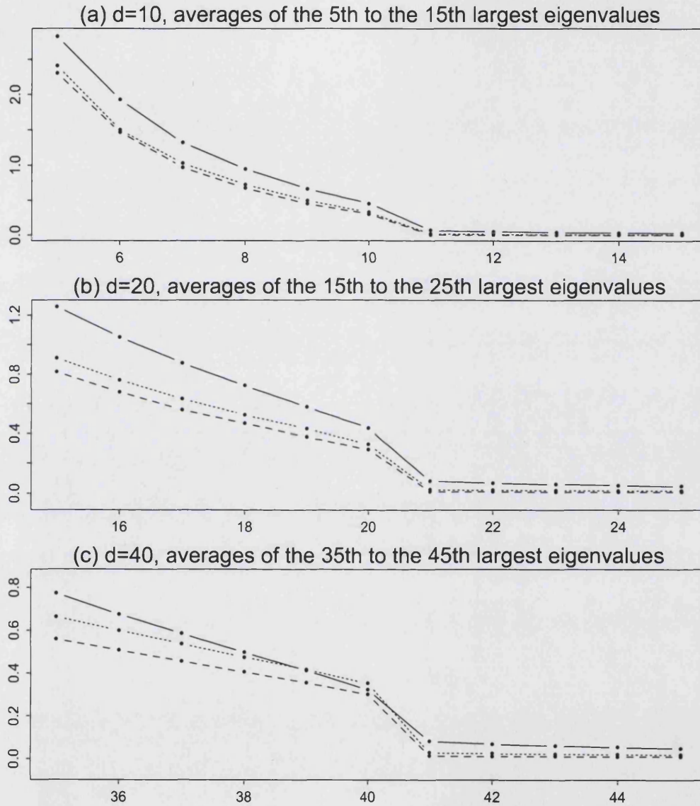
Figure 1.1: The average estimated eigenvalues of the operator \hat{\theta}_j over 200 replications with sample sizes n = 100 (solid lines), 300 (dotted lines) and 600 (dashed lines). Recall that by Proposition 1.1 \theta_j = 0 for all j \geq d + 1 .
