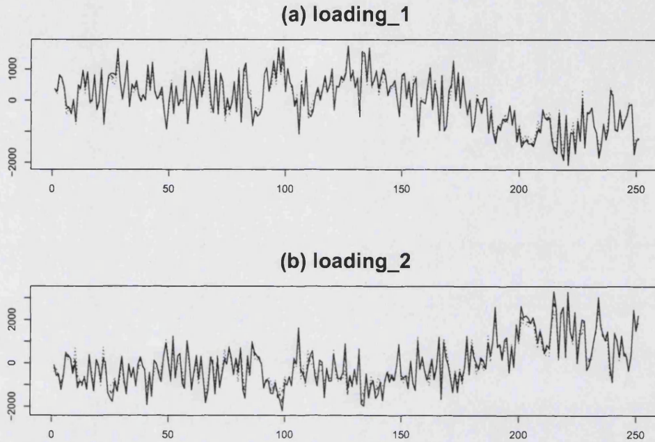
Figure 1.7: Estimated loadings (a) \hat{\eta}_{t1} and (b) \hat{\eta}_{t2} using bandwidths h_t = 0.5\hat{h}_t (solid lines), \hat{h}_t (dashed lines) and 2\hat{h}_t (dotted lines).
