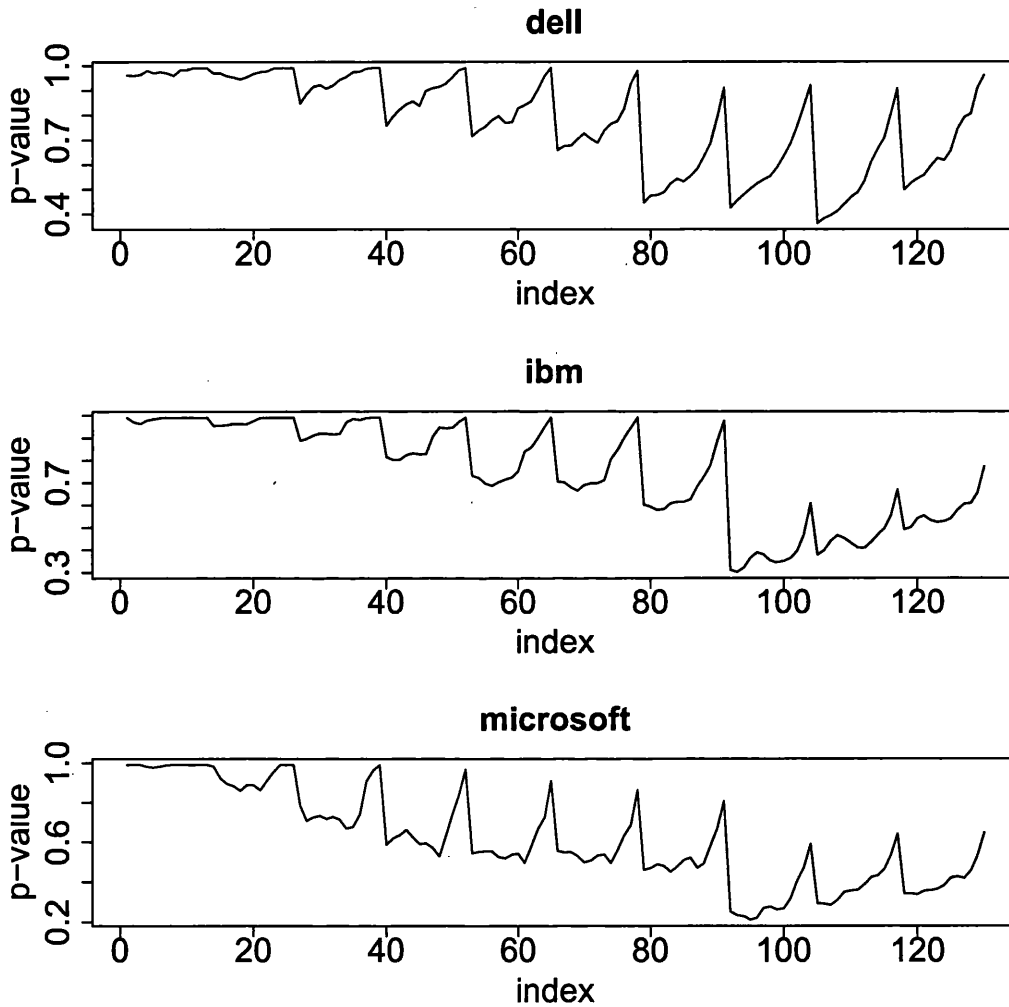
Figure 2.8: P -values from the Dickey-Fuller test for the null H_0 : \delta = 0 in the regression \Delta W_t(u_i, v_j) = \delta W_t(u_i, v_j) + \varepsilon_t . The indices are i = 1, \dots, p_u = 10 and j = 1, \dots, p_v = 13 . Thus the plotted P -values are from a total of p = p_u \times p_v = 130 hypothesis tests.
