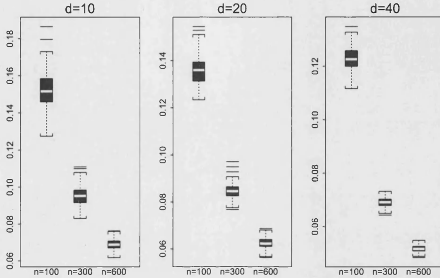
Figure 1.3: Boxplots of the estimated error D'(\hat{\mathcal{M}}, \mathcal{M}) defined in (1.19).
