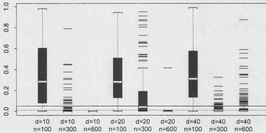
(b) The P-values for testing the (d+1) -th largest eigenvalue
