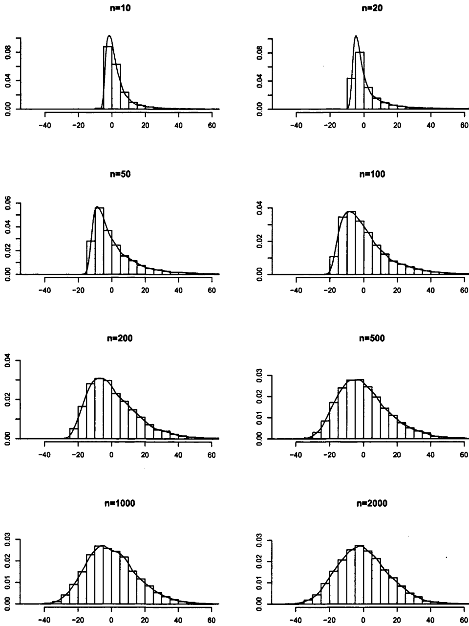
Figure 2.2: Histograms overlaid by kernel density estimates of \sqrt{n}(\hat{\lambda}_1 - \lambda_1) .
