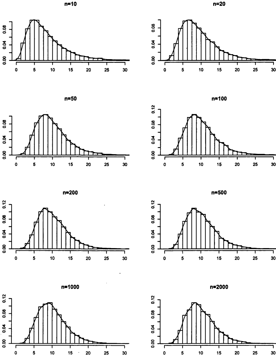
Figure 2.4: Histograms overlaid by kernel density estimates of n\hat{\lambda}_2 .
