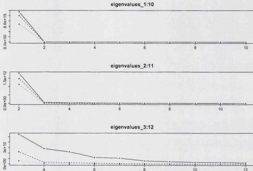
Figure 1.5: Estimated eigenvalues \hat{\theta}_j using bandwidths h_t = 0.5\hat{h}_t (solid lines), \hat{h}_t (dashed lines) and 2\hat{h}_t (dotted lines).
