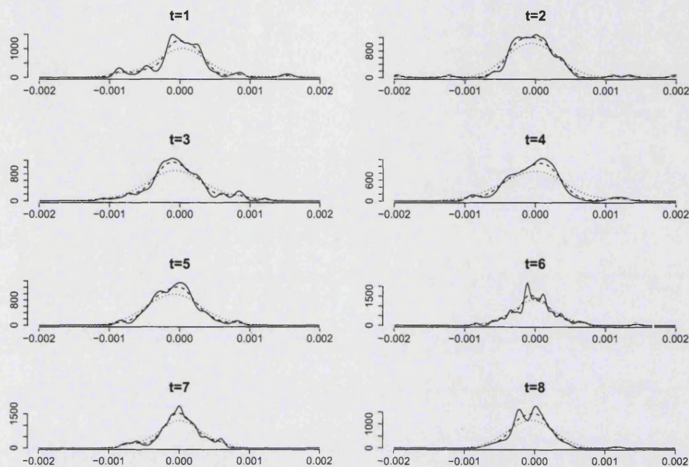
Figure 1.4: Observed densities, Y_t(\cdot) , using bandwidths h_t = 0.5\hat{h}_t (solid lines), \hat{h}_t (dashed lines) and 2\hat{h}_t (dotted lines).
