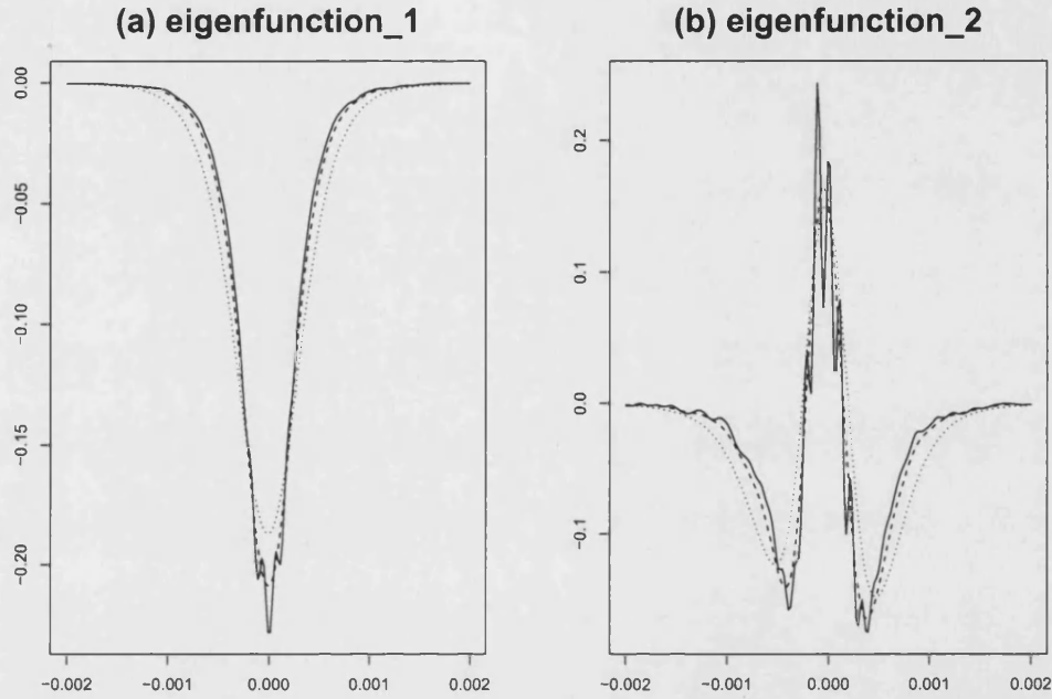
Figure 1.6: Estimated eigenfunctions (a) \hat{\psi}_1 and (b) \hat{\psi}_2 using bandwidths h_t = 0.5\hat{h}_t (solid lines), \hat{h}_t (dashed lines) and 2\hat{h}_t (dotted lines).
