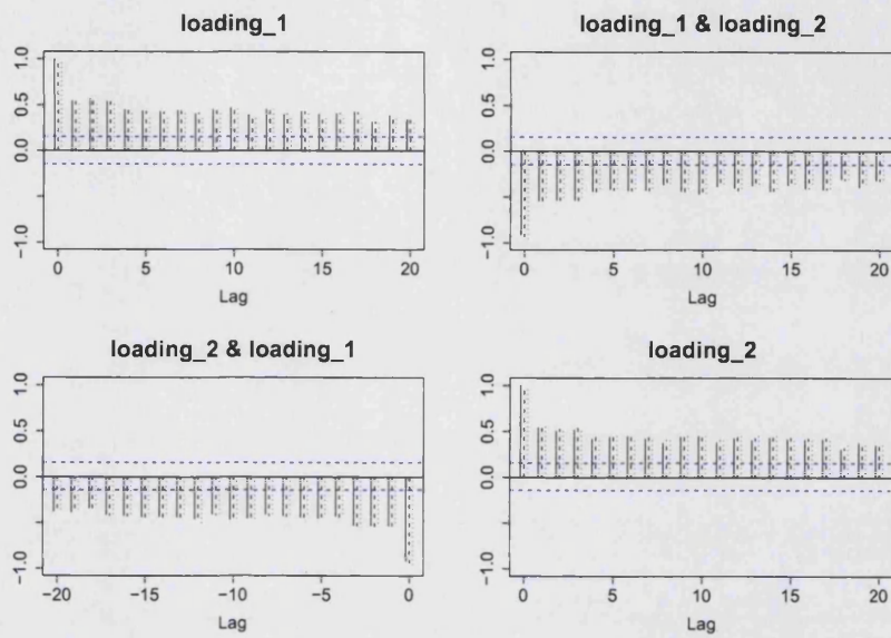
Figure 1.8: ACF of \hat{\eta}_{tj} using bandwidths h = 0.5\hat{h}_t (solid lines), \hat{h}_t (dashed lines) and 2\hat{h}_t (dotted lines).
