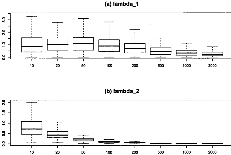
Figure 2.1: Boxplots of estimation errors of eigenvalues; (a) non-zero eigenvalue estimation error |\hat{\lambda}_1 - \lambda_1| and (b) zero eigenvalue estimation error \hat{\lambda}_2 . To add clarity to the display, the outliers are not plotted.
