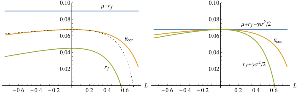
FIGURE 1. \theta_{\text{con}} AND THE UPPER AND LOWER BOUNDS FOR VARIOUS DETERMINISTIC JUMP SIZES L , WITH \gamma = 2 , \sigma = 0.15 , \omega = 0.02 , \mu + r_f = 0.09 . JUMPS ARE BAD NEWS IF L IS POSITIVE AND GOOD NEWS IF L IS NEGATIVE. THE DASHED LINE IN THE LEFT PANEL INDICATES THE MIDPOINT OF THE RISKLESS RATE AND EXPECTED RETURN ON THE RISKY TECHNOLOGY.
