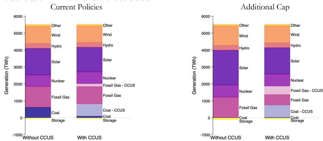
Panel A. Generation mix with and without CCUS
