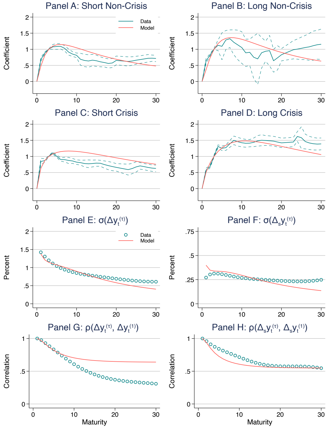
Figure 6: Model Fit
