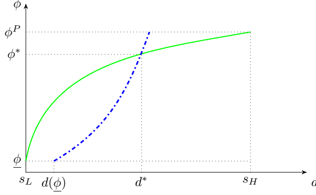
Figure 3: \phi(d) and d(\phi) when E_L s / E_H s < \kappa_P
