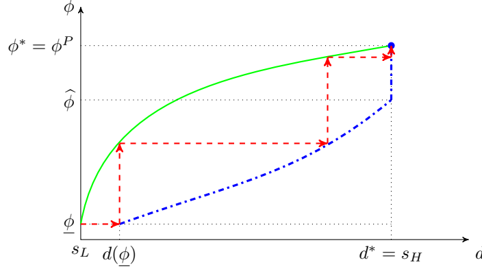
Figure 4: \phi(d) and d(\phi) when E_L s / E_H s > \kappa_P
